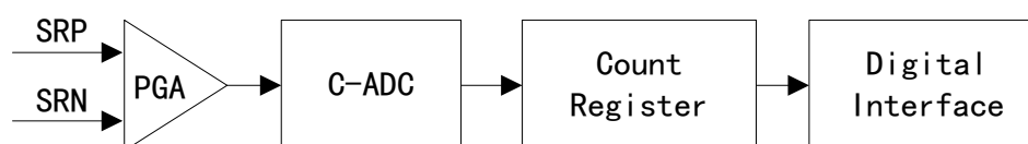
Figure 29 Structure Block Diagram
