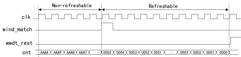
Figure 15 WWDT Timing Diagram
