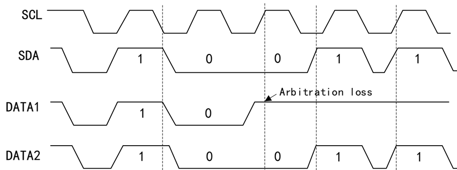
Figure 25 Arbitration Timing
