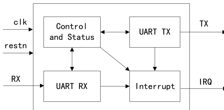
Figure 27 Structure Block Diagram
