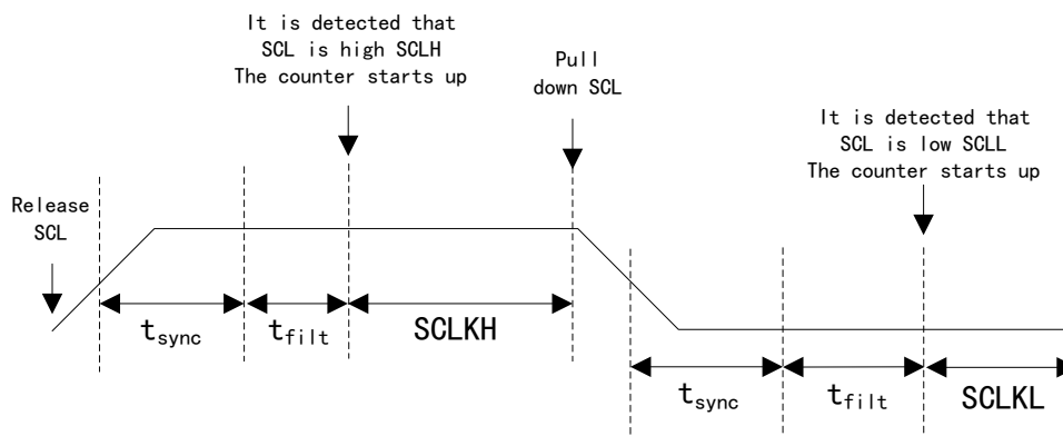
Figure 26 clock Generation
