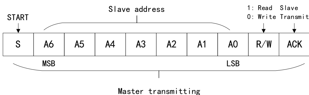
Figure 22 Transmission Address Format
