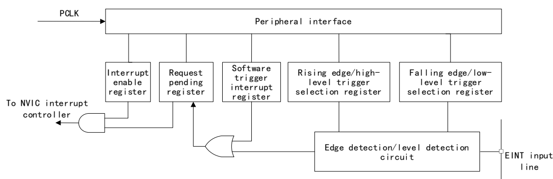
Figure 6 Structure Block Diagram
