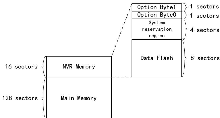
Figure 3 Functional Partitioning of FLASH Regions
