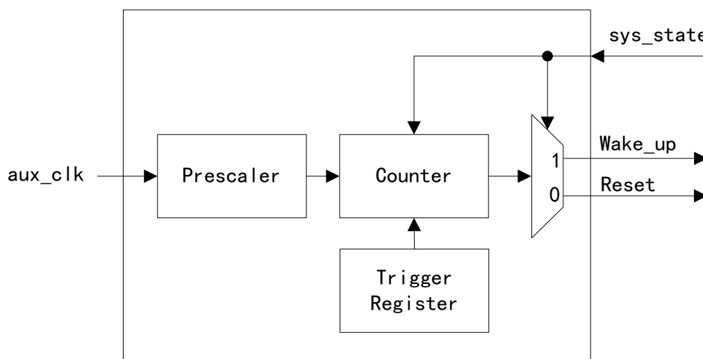
Figure 13 Structure Block Diagram
