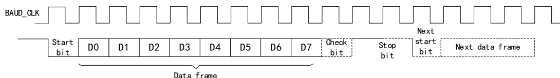
Figure 28 UART Communication Timing
