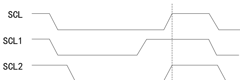
Figure 24 Clock Synchronization
