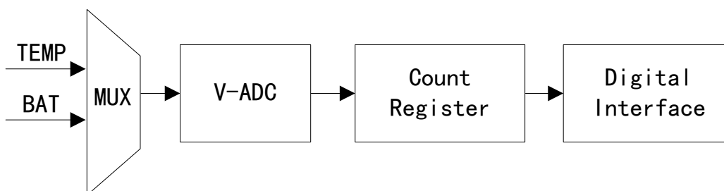
Figure 30 Structure Block Diagram
